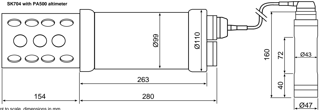
SK704 with PA500 altimeter
